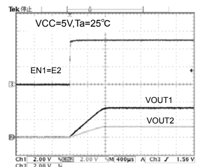
Fig.14 Soft start wave form (Io=0mA)
